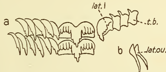
TEXT-FIG. 28.— Armina taniolata . a , As Text-fig. 26 a . \times 105 . b , Two outermost laterals. \times 105 .
